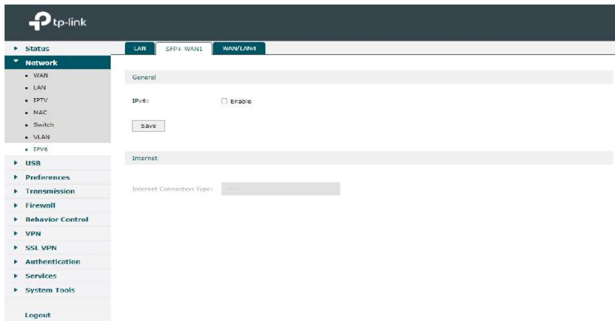
Figure 8-1 Enable IPv6
