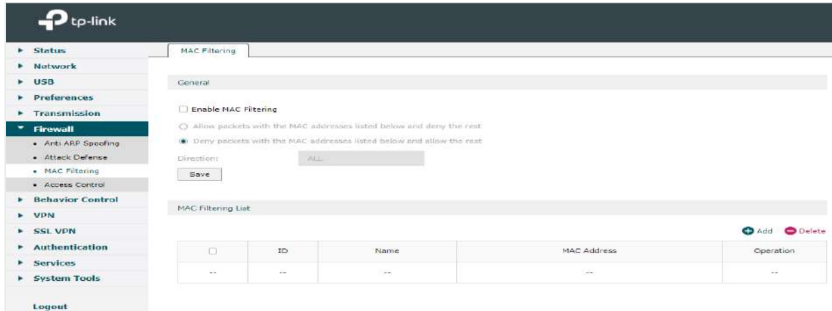
Figure 2-9 MAC Filtering
