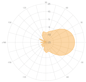
N5-X12 (12 dBi)
