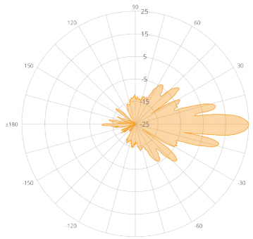
N5-X25 (25 dBi)
