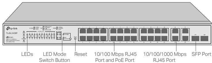
Figure 1-10 Front Panel of TL-SL2428P
