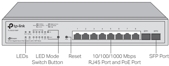
Figure 1-8 Front Panel of TL-SG2210MP
