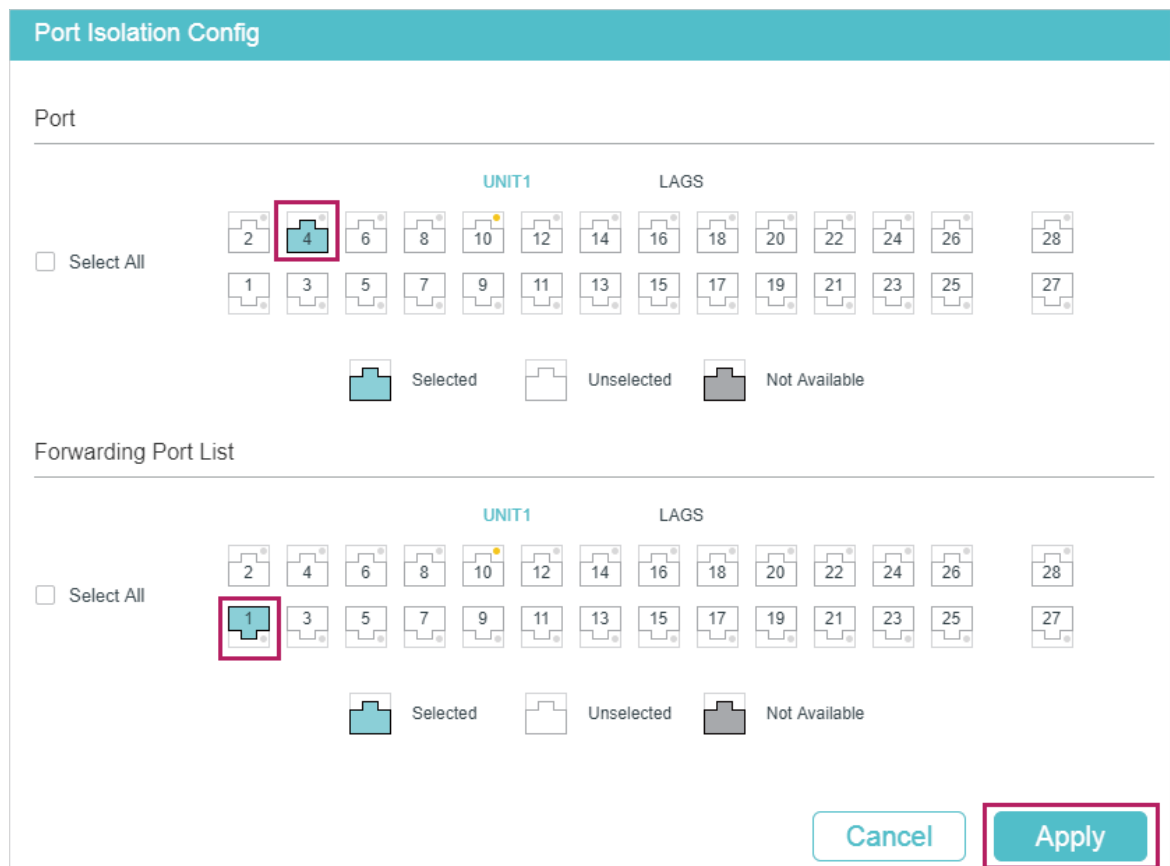
Figure 5-4 Port Isolation Configuration
