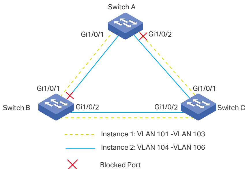
Figure 5-2 VLAN-Instance Mapping
